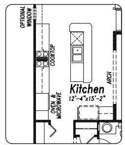
SHOWN WITH OPTIONAL UPGRADED KITCHEN
