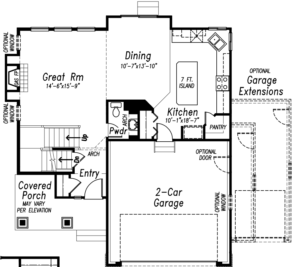
STANDARD 9 FT. CEILINGS Main Level 829 SF
