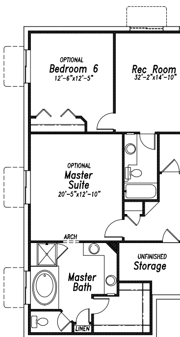
OPT. BASEMENT MASTER SUITE & OPT. BEDROOM 6
