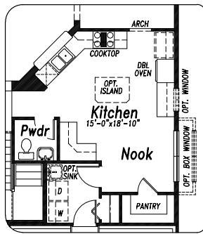
OPT. DBL OVEN KITCHEN LAYOUT
