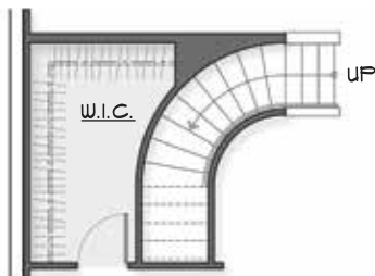
Optional Curved Stair
